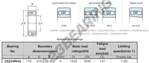
Boundary dimensions
