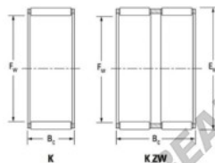
Backed needle roller and cage assemblies
