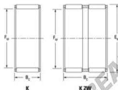
Radial inducte roller and cage assemblies
