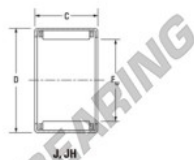
Boundary dimensions
