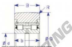
D Double Row Style IV Roller Bearing
